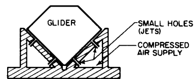
Fig. 10-1. End view of linear air trough.
